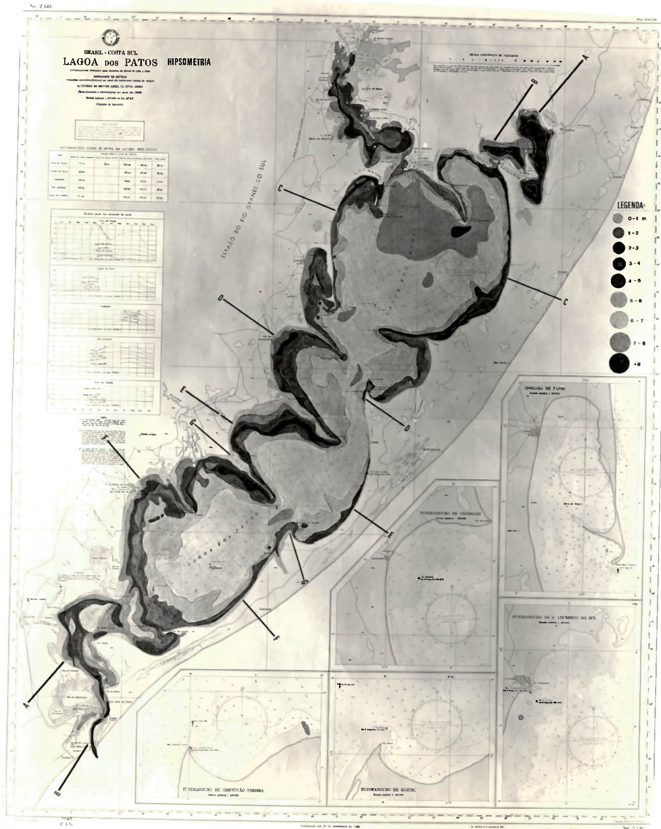
Fig. II.17 - Bathy-hipsometric map of Lagoa dos Patos, indicating the vertical profile orientation (DHN Nº 2140).
